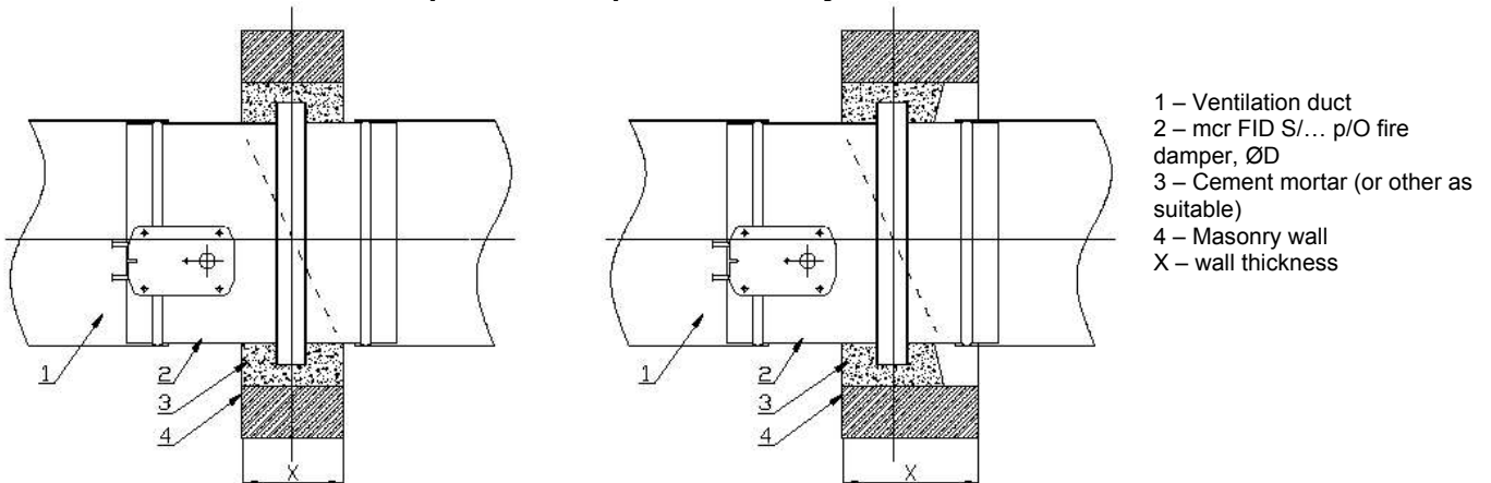
Installation of the mcr FID S/... p/O fire damper in masonry and concrete walls
